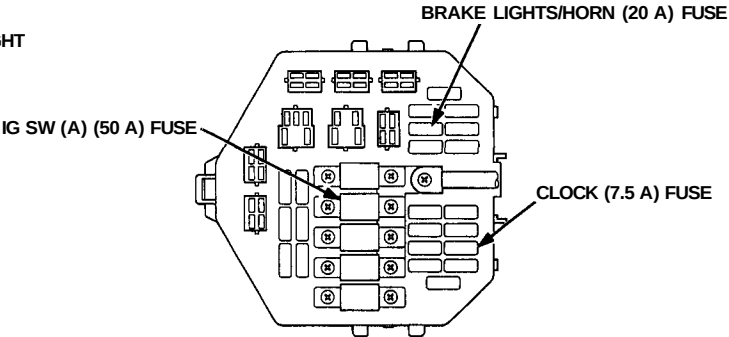
UNDER-HOOD FUSE/RELAY BOX
